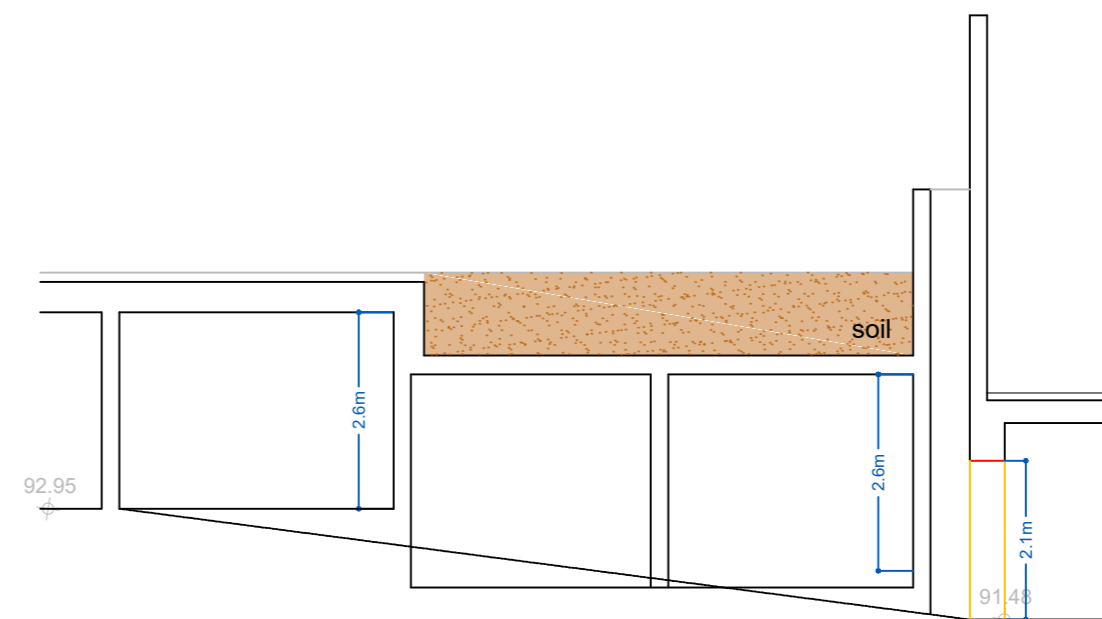
part section x-x through ramp
